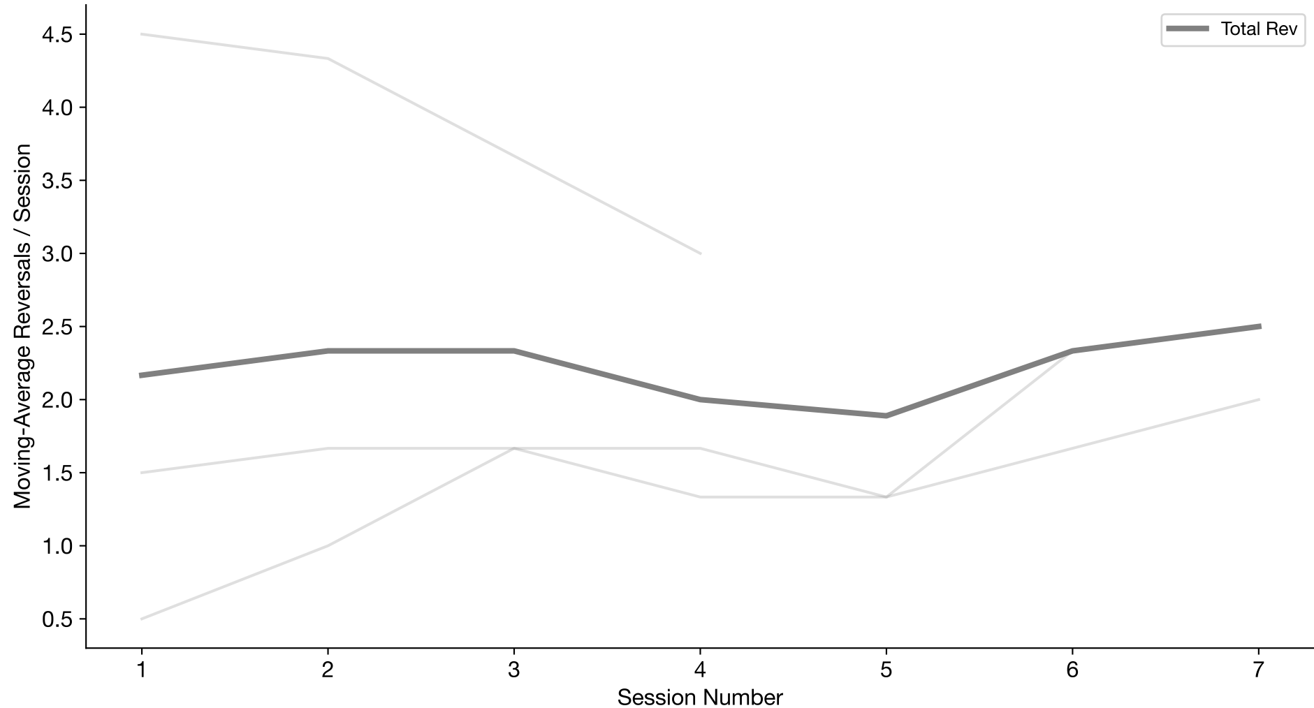
Moving-Average Total Reversals Over Time (n=3 subjects; sessions per subject=4-7; window=3)
